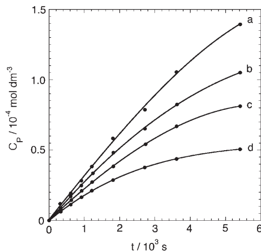
Fig. 8. Time dependence of concentration of produced 4-nitrophenol catalyzed by free phosphatase for the initial substrate concentration of 5 \times 10^{-4} mol dm ^{-3} (a), 2 \times 10^{-4} mol dm ^{-3} (b), 1 \times 10^{-4} mol dm ^{-3} (c), and 8 \times 10^{-5} mol dm ^{-3} (d). The pH of the solution was 4.8.
