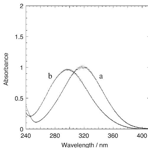
Fig. 2. Absorption spectra of 1 \times 10^{-4}\text{ mol dm}^{-3} 4-nitrophenol and 1 \times 10^{-4}\text{ mol dm}^{-3} 4-nitrophenyl phosphate in 0.1\text{ mol dm}^{-3} acetate buffer solution (pH = 4.8), which contained 0.1\text{ mol dm}^{-3} NaCl: 4-nitrophenol (a); 4-nitrophenyl phosphate (b).
