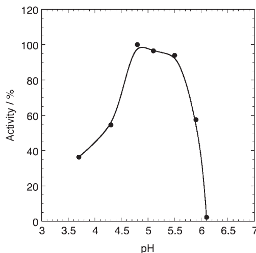
Fig. 7. The pH dependence of the flux of 4-nitrophenol produced during the hydrolysis of 4-nitrophenyl phosphate using the immobilized enzyme. Activities (%) relative to the flux at pH 4.8 are plotted as a function of the pH in the solution. The 0.1 mol dm ^{-3} buffer and 0.1 mol dm ^{-3} NaCl were included in the substrate solution. The initial concentration of 4-nitrophenyl phosphate in the external solution was 5 \times 10^{-3} mol dm ^{-3} .
