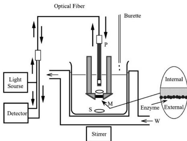
Fig. 1. Schematic diagram of assembled system for the measurement of 4-nitrophenol amount transported through the enzyme membrane. The time dependence of the amount of phenol in the internal solution was obtained through the measurement of the absorption spectrum using an immersed probe (P) connected to a fiber UV spectrophotometer. The arrow ( \longrightarrow ) shows the path of the ultra-violet radiation. Immobilized-enzyme membrane, magnetic spin bar, and thermostatically controlled water are designated by M, S, and W, respectively.
