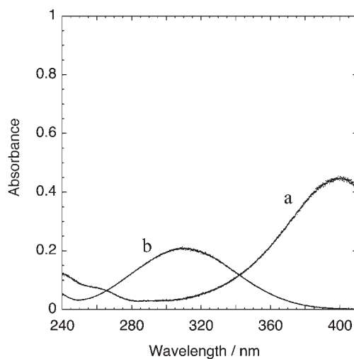
Fig. 3. Absorption spectra of 2 \times 10^{-5}\text{ mol dm}^{-3} 4-nitrophenol and 2 \times 10^{-5}\text{ mol dm}^{-3} 4-nitrophenyl phosphate in 0.1\text{ mol dm}^{-3} Tris buffer solution (pH 8.5), which contained 0.1\text{ mol dm}^{-3} NaCl: 4-nitrophenol (a); 4-nitrophenyl phosphate (b).
