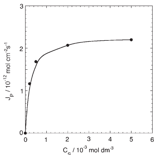
Fig. 6. Concentration dependence of flux across the enzyme membrane at pH 4.8. The flux of 4-nitrophenol produced during the hydrolysis of 4-nitrophenyl phosphate using immobilized enzyme was determined by measuring the absorption spectra of the internal solution. The initial concentration of 4-nitrophenyl phosphate was in the range of 2 \times 10^{-4} mol dm ^{-3} – 5 \times 10^{-3} mol dm ^{-3} . 0.1 mol dm ^{-3} acetate buffer (pH 4.8) and 0.1 mol dm ^{-3} NaCl were included in the substrate solution.
