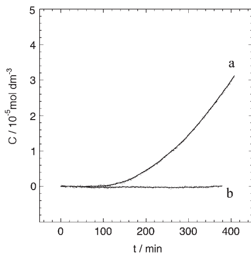
Fig. 4. Time course of the concentration in the internal solution for 4-nitrophenol (a) and that for 4-nitrophenyl phosphate (b). Two compartments are separated by the perfluorocarboxylate ionomer membrane without enzyme. Initially, both the external and the internal solutions contained 0.1 \text{ mol dm}^{-3} acetate buffer (pH 4.8) and 0.1 \text{ mol dm}^{-3} NaCl. Initial concentration in the external solution of 4-nitrophenol or that of 4-nitrophenyl phosphate was 0.01 \text{ mol dm}^{-3} .
