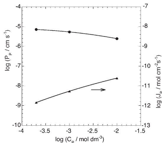
Fig. 5. The membrane permeability of the perfluorocarboxylate ionomer membrane in the absence of the enzyme. The membrane permeability to 4-nitrophenol, P_P , and the flux of 4-nitrophenol, J_P , are shown as a function of the initial concentration of 4-nitrophenol in the external solution.
